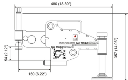
Maximum extension BFA4TM in mm (inch)
