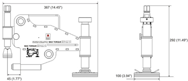
Minimum extension BFA4TM in mm (inch)
