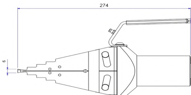
Tool Dimensions - Closed
