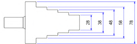
Safety Block (Part No. B1095) Dimensions
